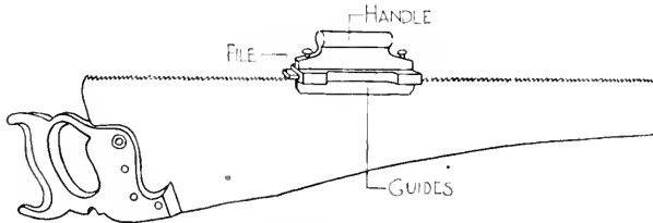
FIG. 108. TOP JOINTING A SAW.
